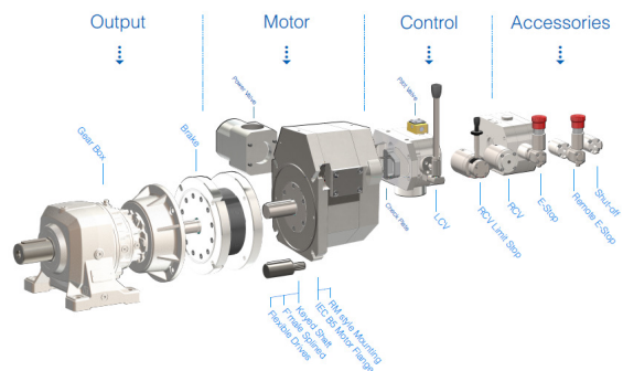
ARMAX Geared Piston Motors GP
